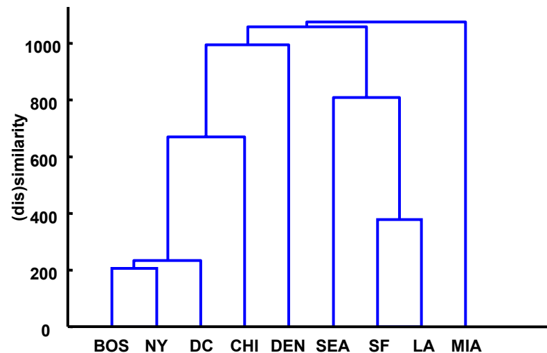
Single-linkage
