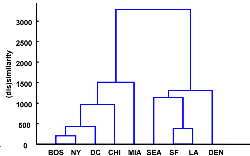
Complete-linkage
